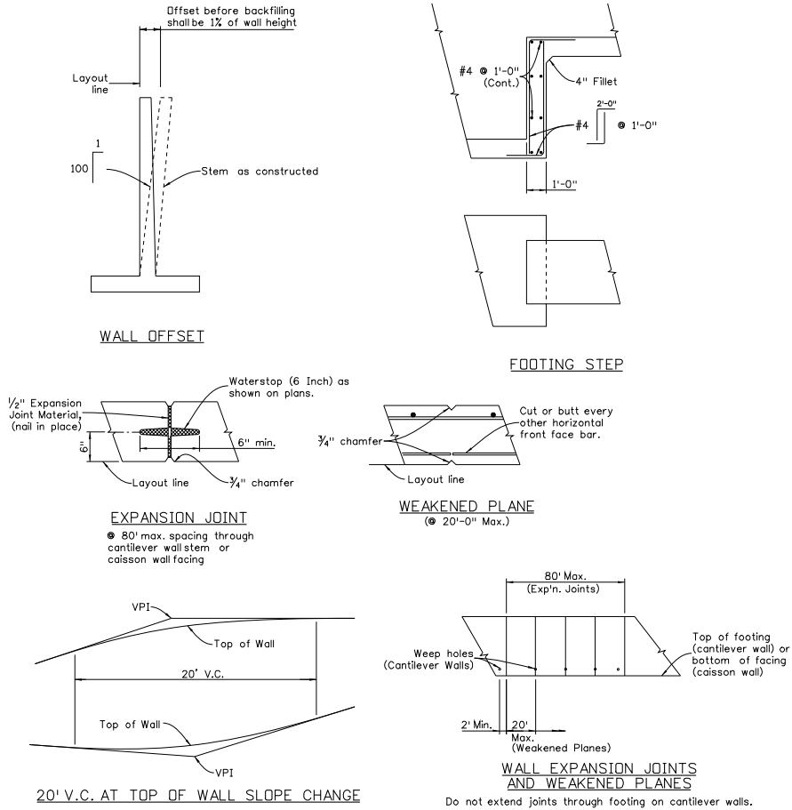
Fig. 15.1.9-3 Cast In Place Details
